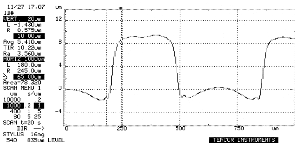
Fig. 4 Profile measurement of commercial retarder stripes.
