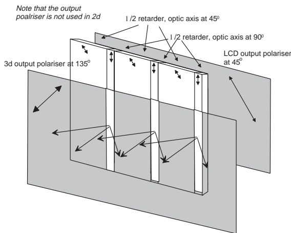
Fig. 3 Retarder Prallax barrier configuration.
