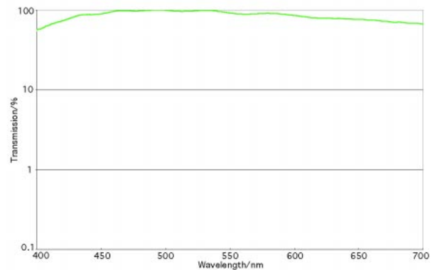
Fig. 5 Transmission of RM retarder.
