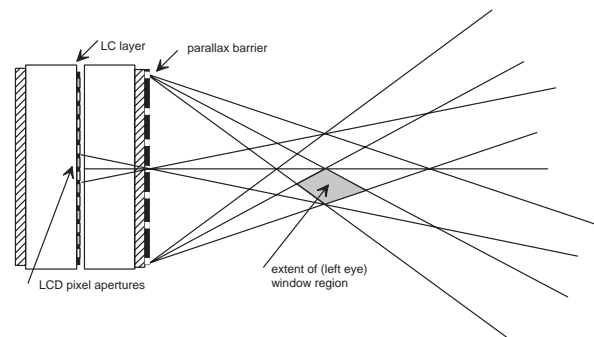
Fig. 2 Parallax barrier LCD display.
