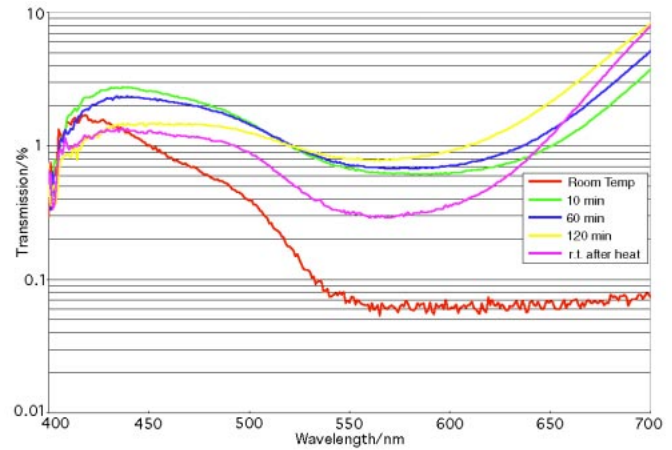
Fig. 7 Standard iodine polariser in extinction, heating to 140 °C.
