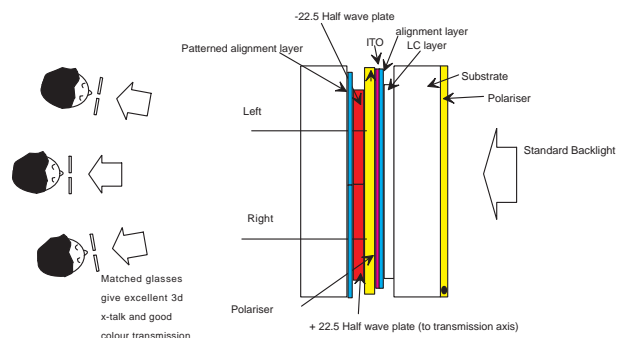
Fig. 8 Internal polariser 3d display.
