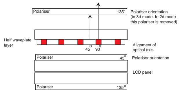
Fig. 6 2d/3d display configuration.
