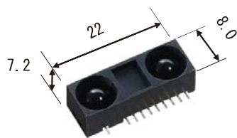
従来品 (GP2Y0A60SZ0F)
